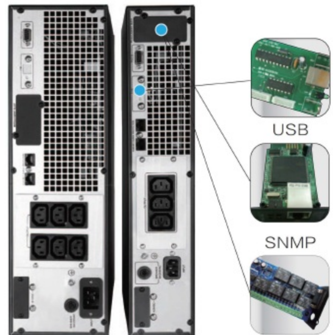
Drycontact board
